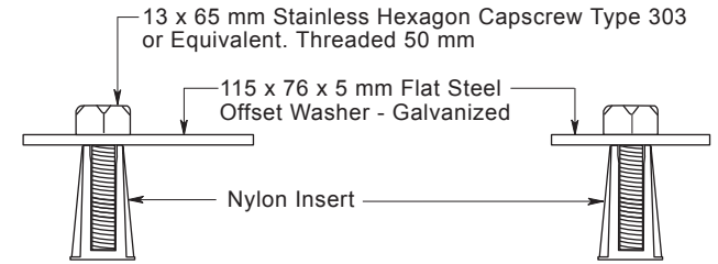
FASTENER DETAIL
